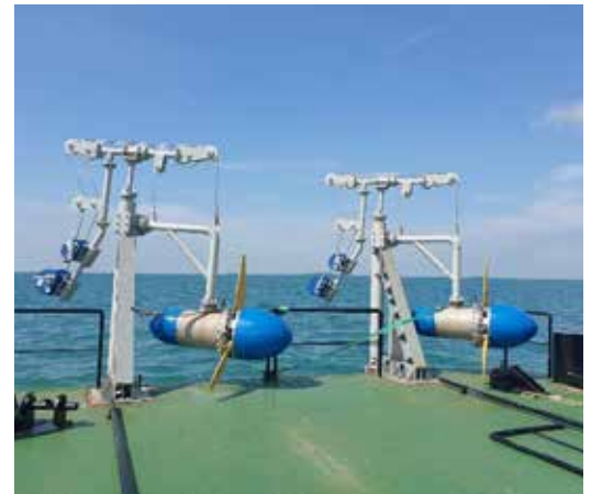
Figure 2: Turbines hoisted out of the water for maintenance.
