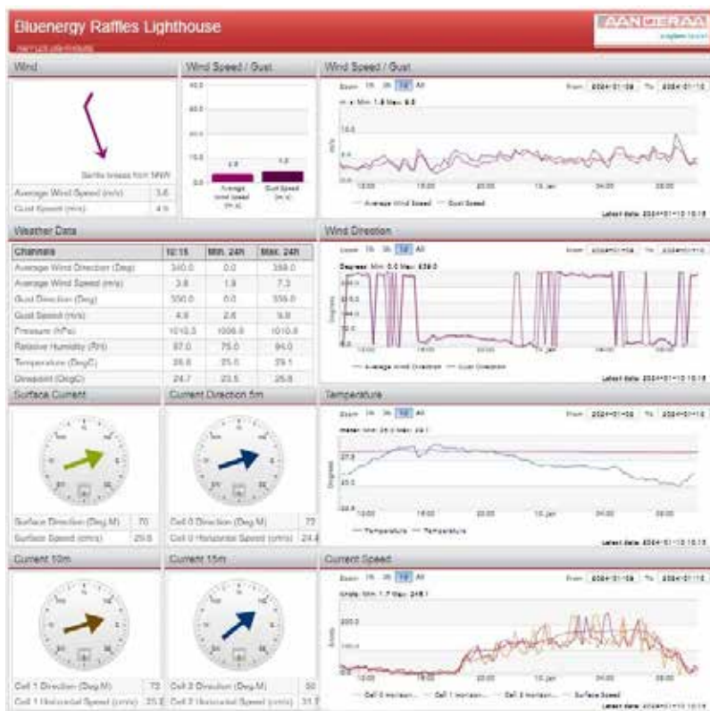
Figure 5: Screenshot of real time current and meteorological parameters displayed in Geoview IoT hosted by Aanderaa in Norway.
