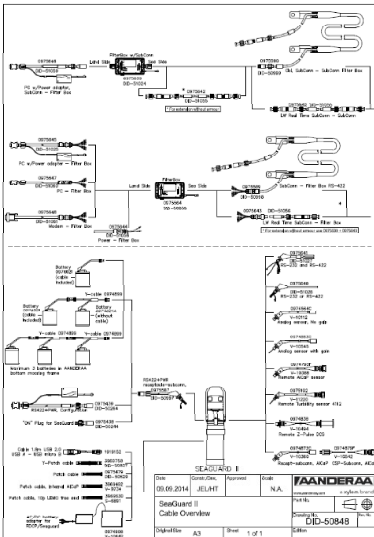
Figure 4-6: SeaGuardII cable overview
