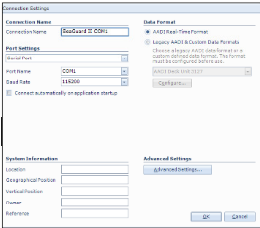
Figure4-2 Connection via Serial Port
