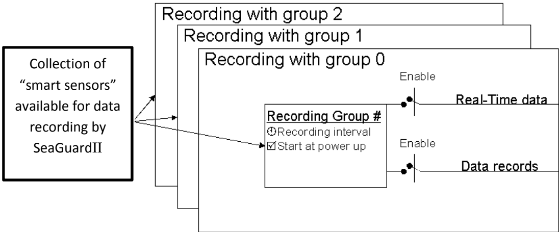
Figure 3-10 Recording group structure
