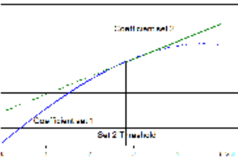
Figure 5-8 Two polynomials analog sensor
