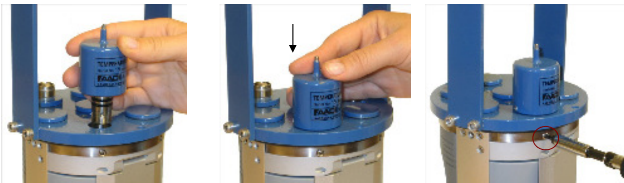
Figure7-11 AiCaP sensors: Place the sensor according to the orientation pin. Push down the sensor and fasten the set screw.
