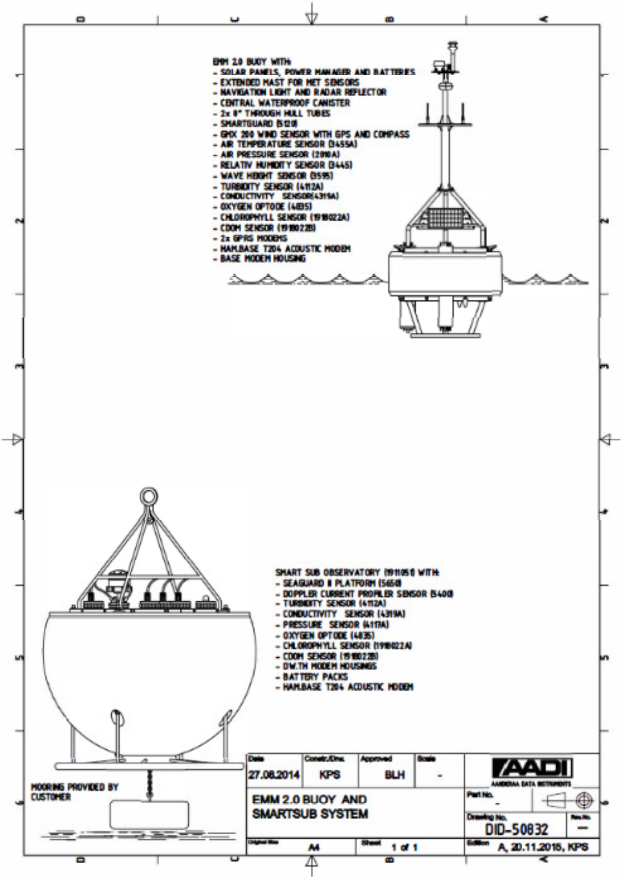
System drawing DID-50832
