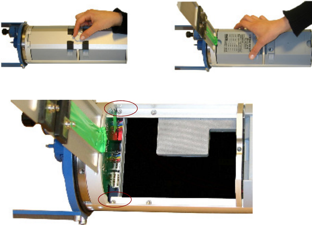
Figure7-12 Open the battery lid, remove the upper battery, and unscrew the two top screws that holds the top front cover. Turn the instrument and pull off the top front cover.
