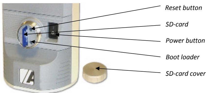
Figure 1- 3 SD-card slot
