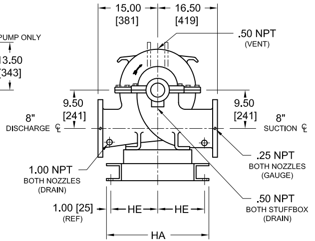
CW ROTATION VIEWED FROM COUPLING END
