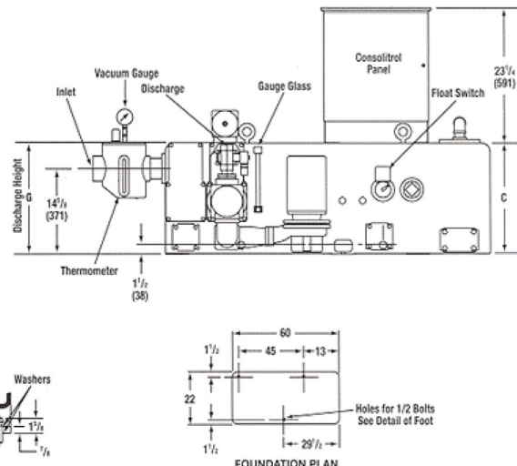
100 GAL (379L) RCVR
