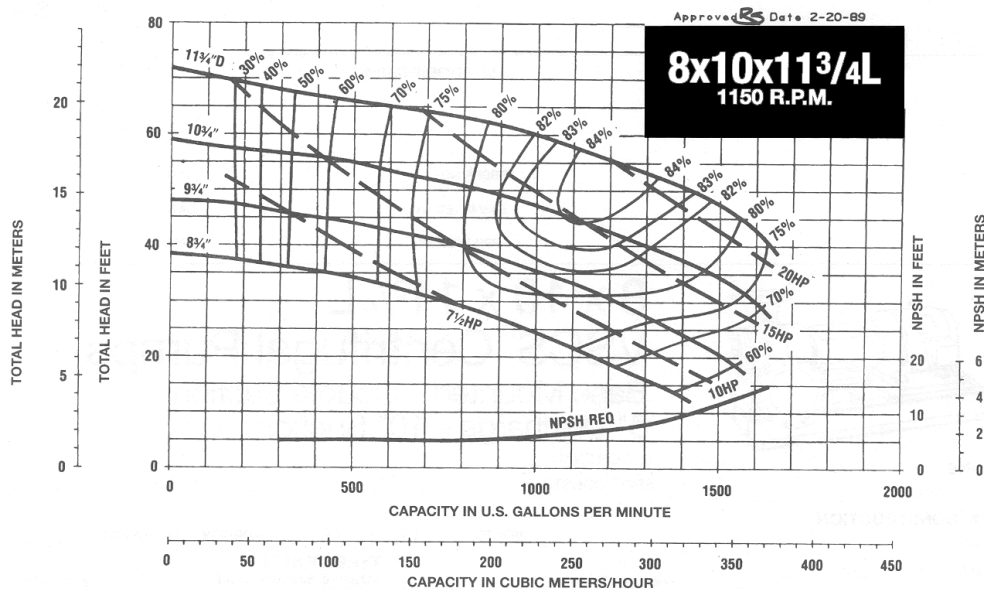
PERFORMANCE CHARACTERISTIC CURVE
