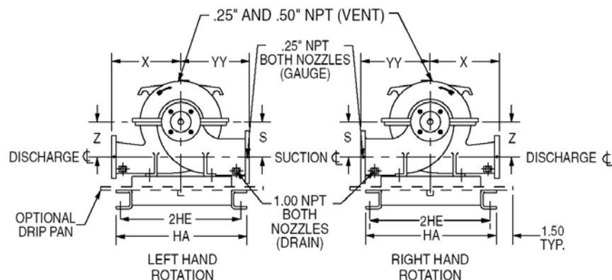
FLANGE DIMENSIONS IN INCHES
