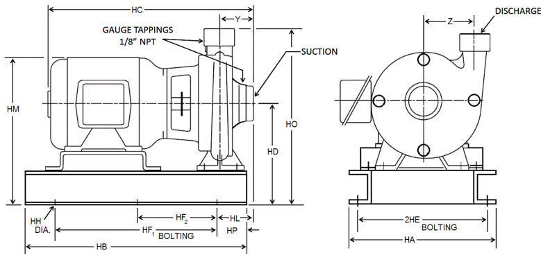
DIMENSIONS - INCHES (mm)
