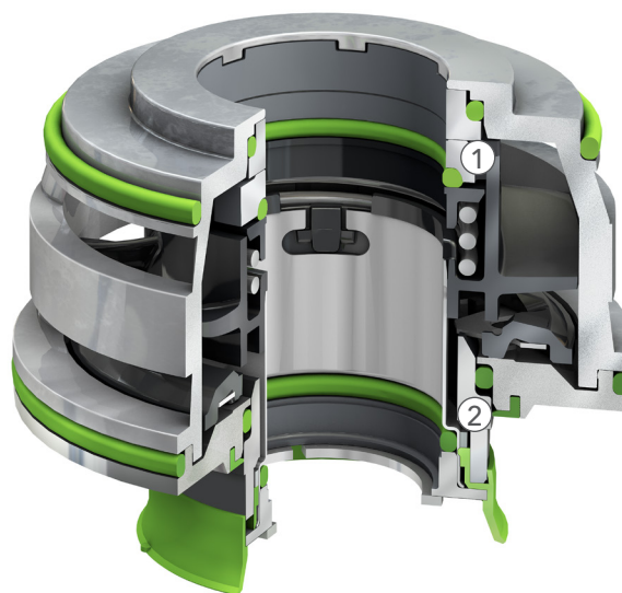
Plug-in Seal with the Active Seal system.
