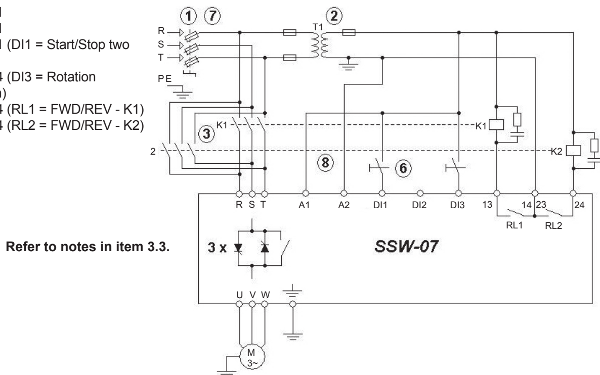
Figure 3.12 - Recommended Set-up with Command via Two-wire Digital Inputs and Direction of Rotation
