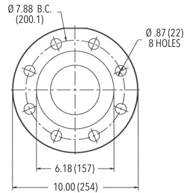
316SS 4\" Class 300 R.F. (1 - 6 Stages) Optional
