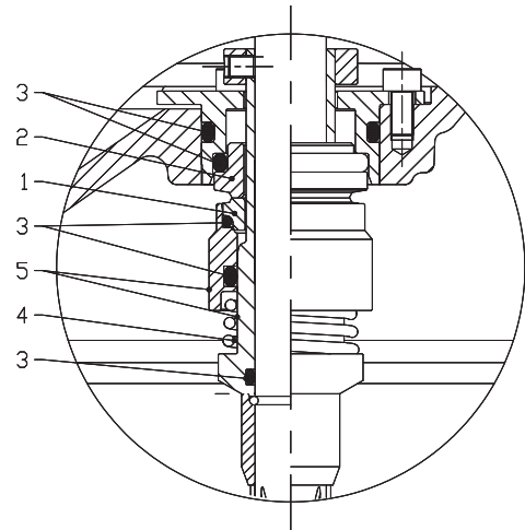
Balanced cartridge seal
