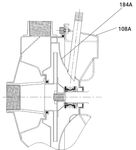
Seal face vent/flush option
