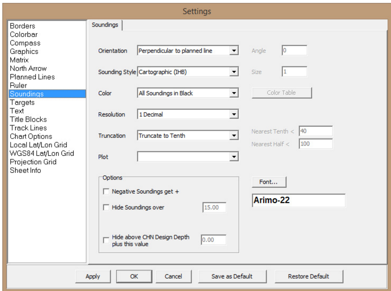
FIGURE 3. Fig 3: The Soundings Setting of the Control Panel
