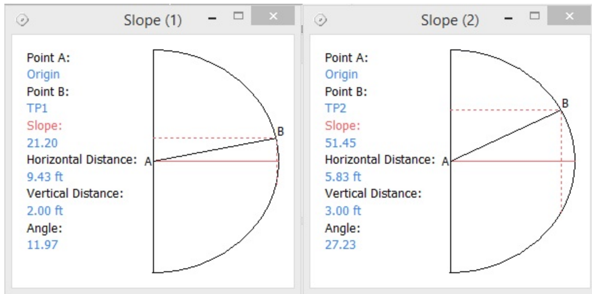
FIGURE 4. SURVEY program running with a couple of Tracking Slope Windows
