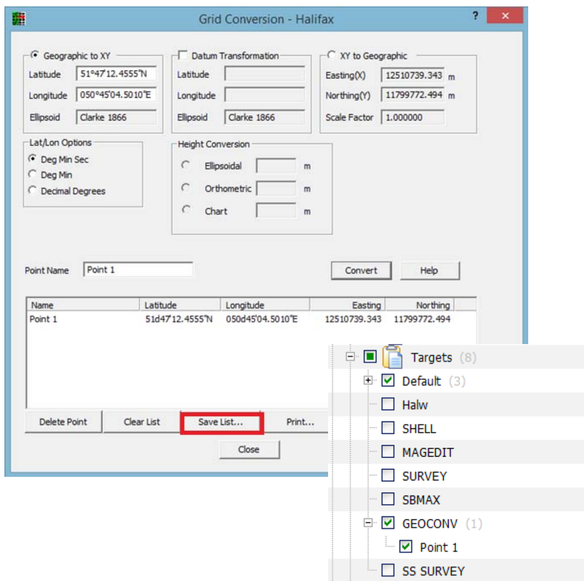
FIGURE 1. Click [Save List...] to Send to The Target Database—GRID CONVERSION (left) and The New Target Listed in the Shell (right).
