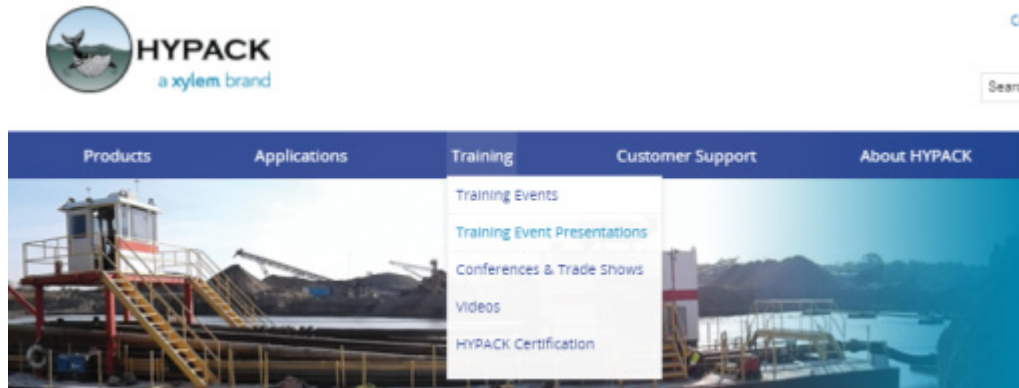
FIGURE 4. Training Menu
