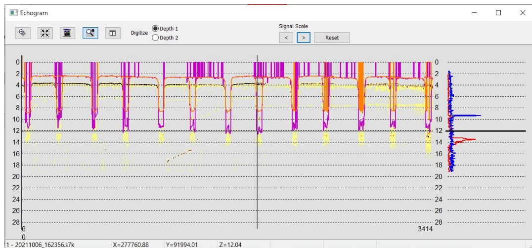
Figure 4: Echogram from .S7K file
