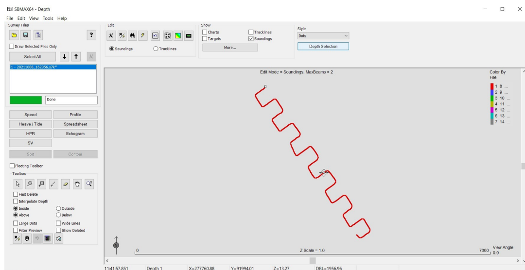
Figure 2: Soundings from .S7K File, Dot Display
