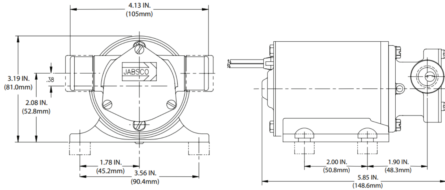
DIMENSIONAL DRAWING INCHES (MILLIMETRES)
