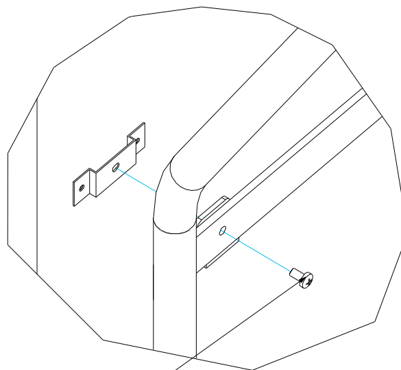
M5 Fixing Screw
