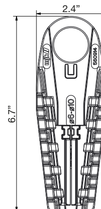
Mounting bracket for MJK Expert™ 1400 level transmitter
