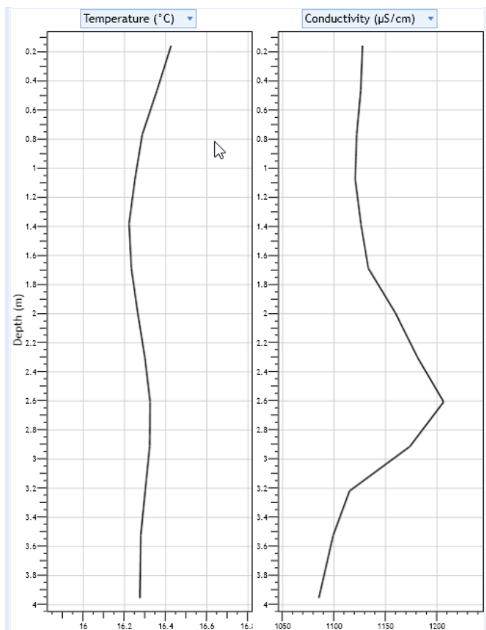
Figure 12: Bioreactor 1 CTD Measurement.
