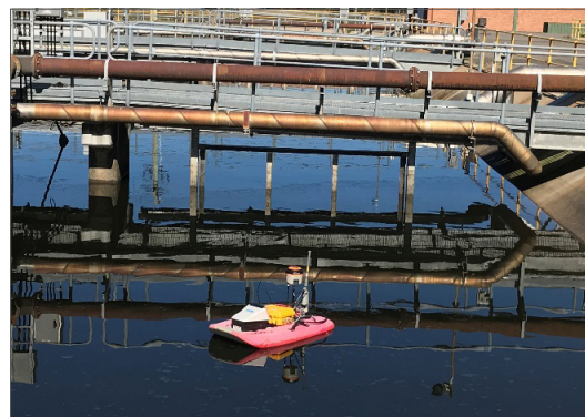
Fig. 4. Autonomous rQPOD.
