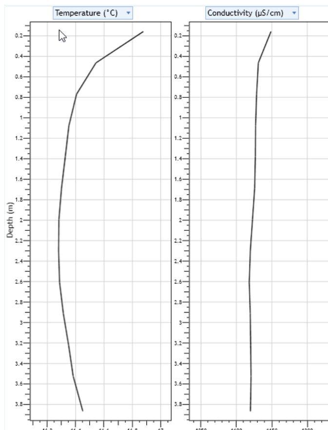
Figure 13: Bioreactor 2 CTD Measurement.
