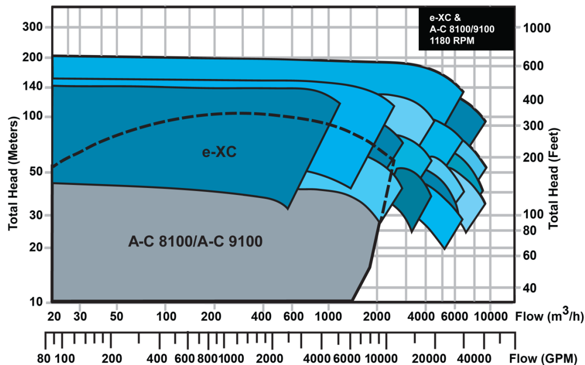
60 Hz – e-XC & AC 8100/AC 9100, 1180 rpm
