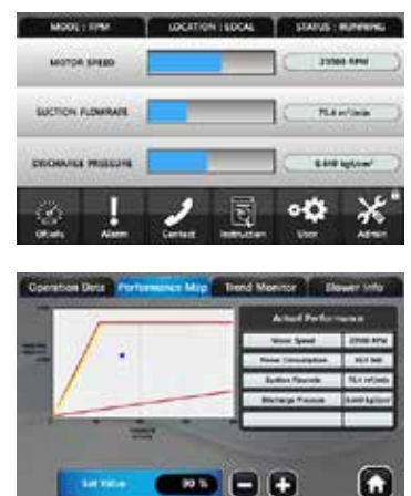
Sample HMI screens and settings for TurboMAX
