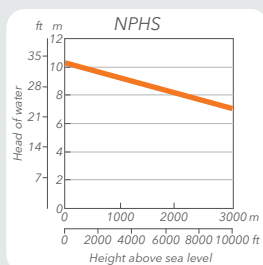
Air pressure in head of water at different heights.
