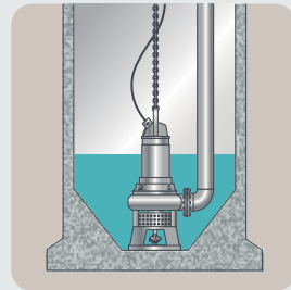
Pump with agitator
