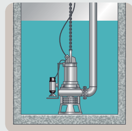
Pump with side-mounted mixer
