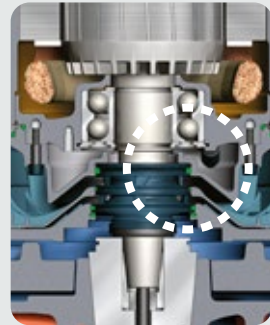
Inspection chamber, 5100/5150
