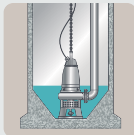
Pump with internal cooling system
