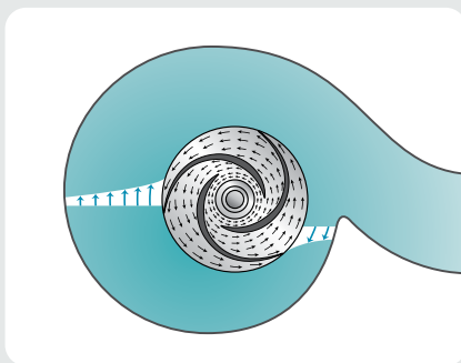
Flygt hydraulic design reduces slurry velocity
