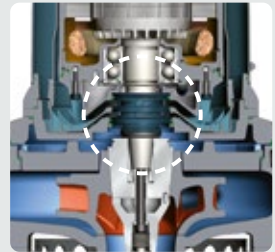
Plug-in™ seal (5100/5150)
