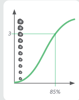
Sieve curve
