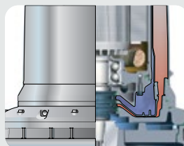
Pump with internal cooling system
