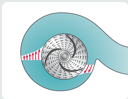
Standard hydraulic design makes slurry move at high velocity
