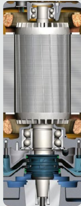
Pump shaft and bearings
