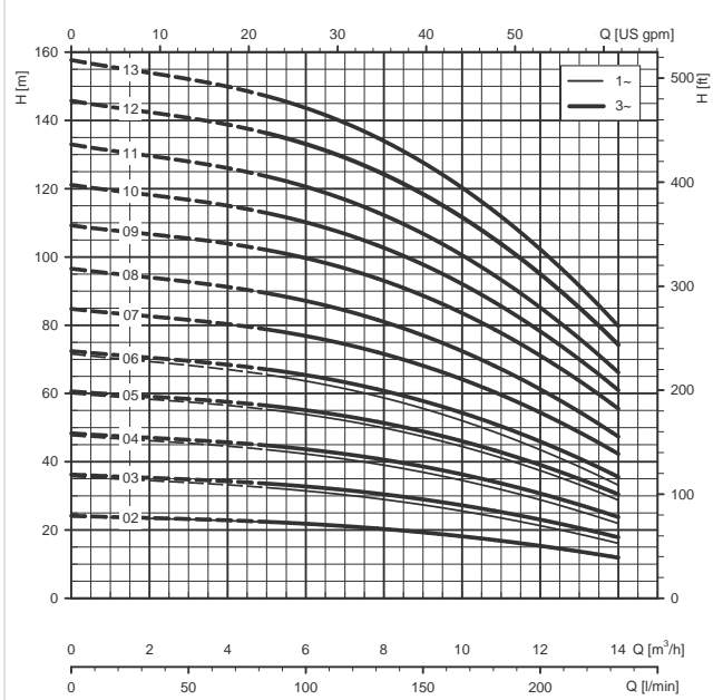
↳ 10HM..S - 10HM..N SERIES OPERATING CHARACTERISTICS AT 50 Hz, 2 POLES
