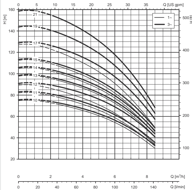
↳ 5HM..S - 5HM..N SERIES, (10 TO 21 STAGES) OPERATING CHARACTERISTICS AT 50 Hz, 2 POLES
