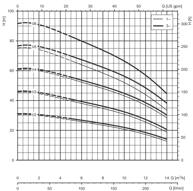
↳ 10HM..P SERIES OPERATING CHARACTERISTICS AT 50 Hz, 2 POLES
