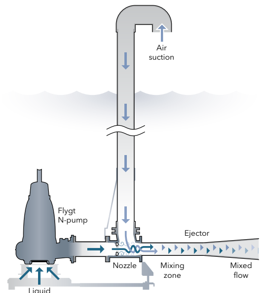
Working principle; The velocity of the water creates air suction which is mixed in the ejector and transferred into the wastewater tank.
